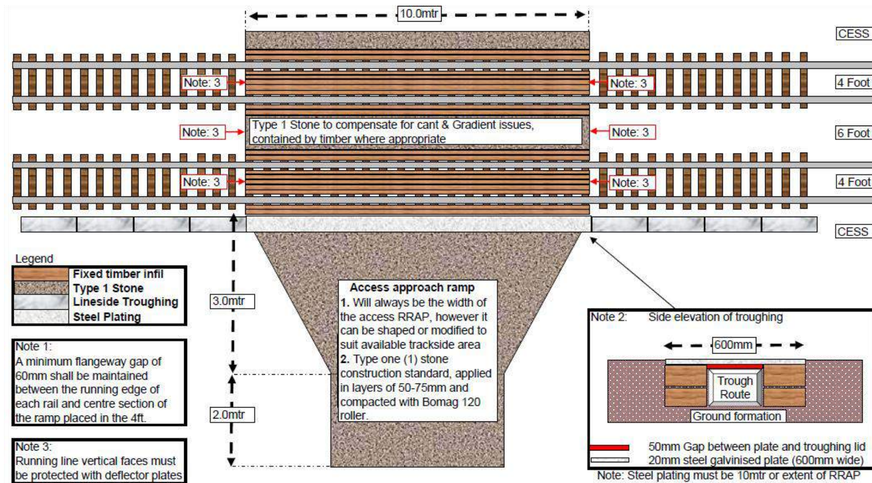
Figure 3 Construction type C
