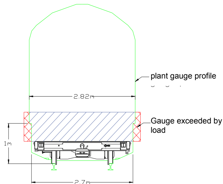
Figure 10 Illustration of load exceeding plant gauge
