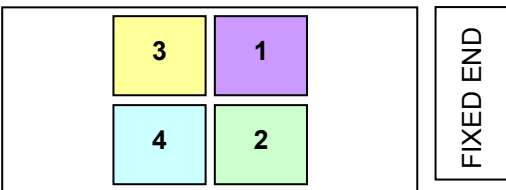
Figure 7 Alternative loading sequence for a partial loads
