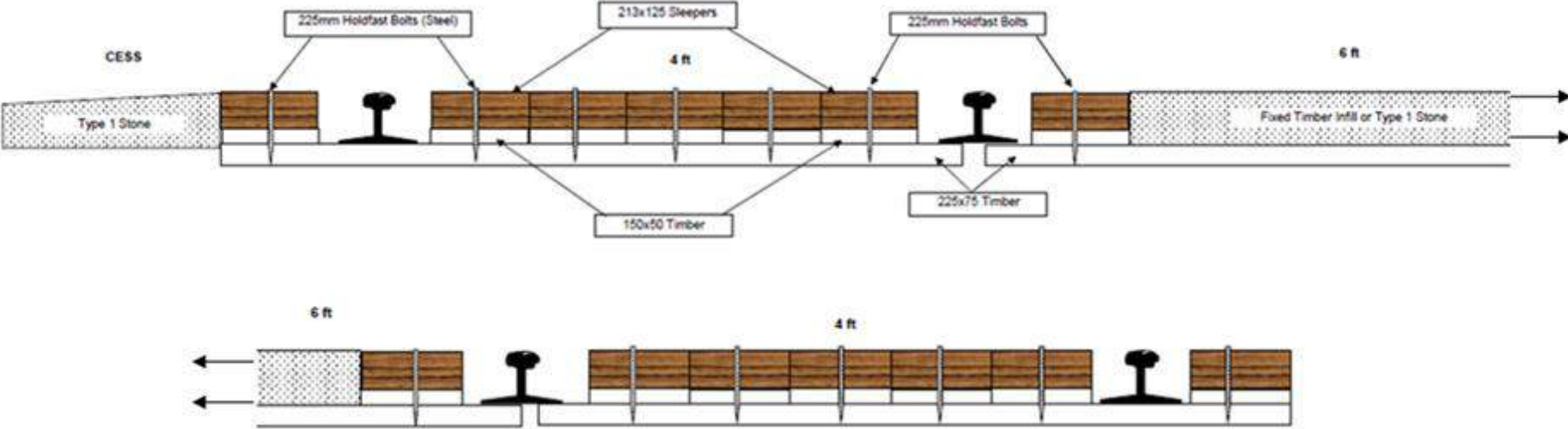
Figure 6 Fixed timber infill (side elevation)
