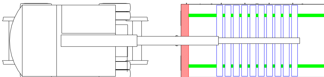
Figure 8 Loading a trailer with limited load/outreach capacity
