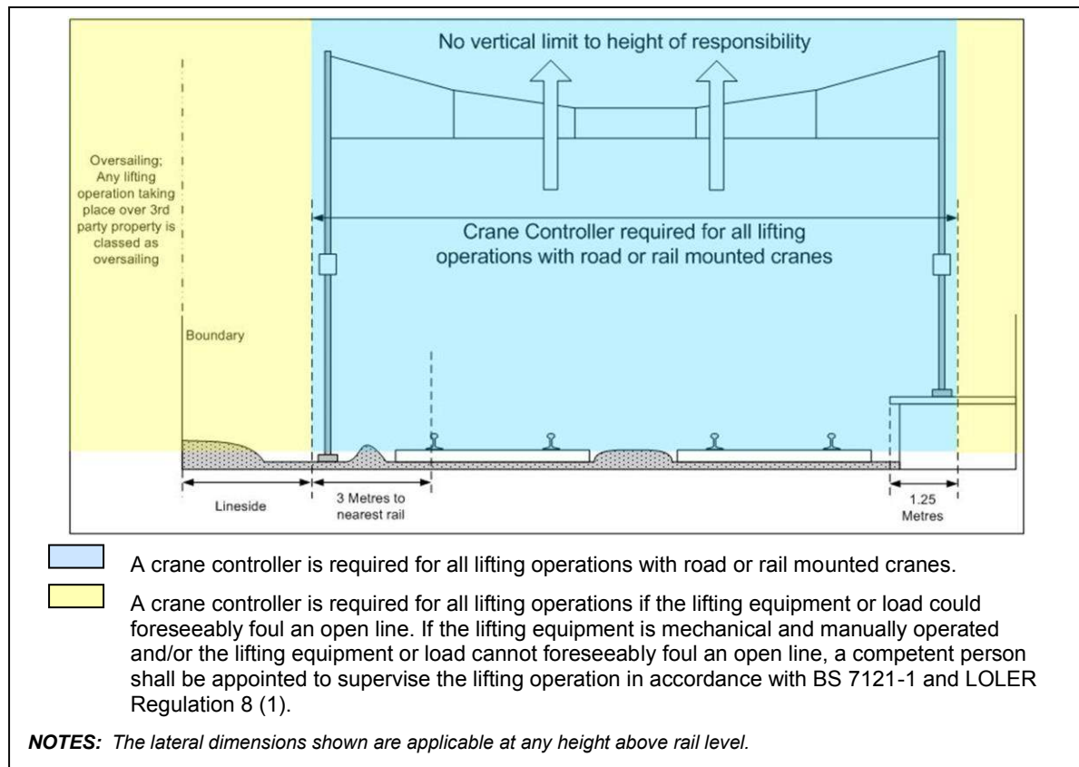
Figure 1 When a Crane controller is required
