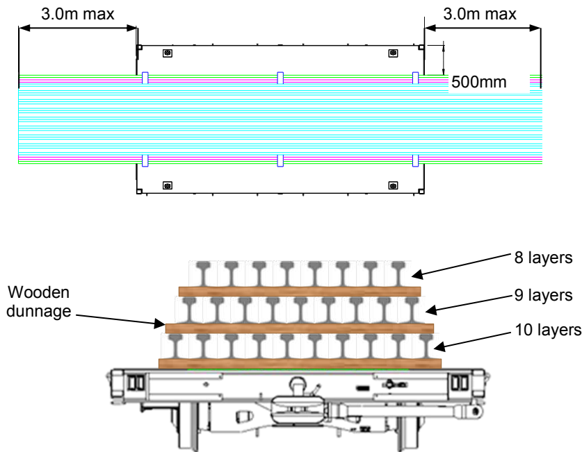
Figure 3 Carrying '30ft' rails
