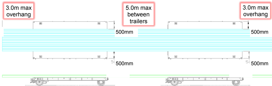
Figure 3 Carrying '30ft' rails
