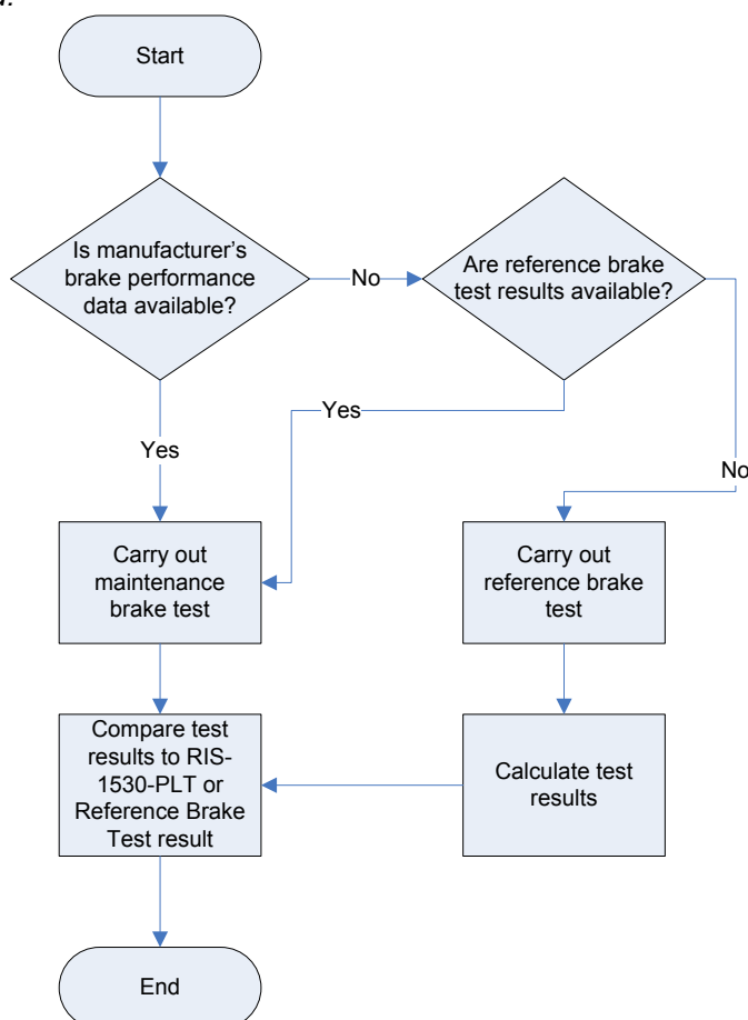
Figure 1 - Road-rail vehicle brake testing process
